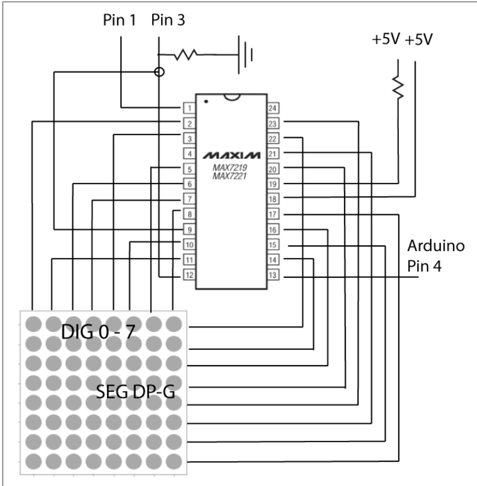
Figure 11-19. Maxim7221 schematic
